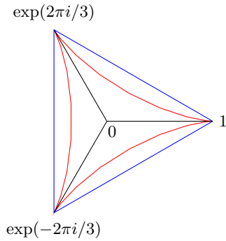
Figure 6.2.: Instantons in the complex \psi plane. The nodes correspond to the four SU(3) -instantons on the nearly Kähler manifold M^6 , whereas the edges are interpolating Spin(7) -instantons on M^8 = cyl(c(M^6)) or submanifolds thereof. The blue edges can be realized as G_2 -instantons on the cocalibrated cylinder cyl(M^6) , the red ones solve the nearly parallel G_2 -instanton equation on the sine-cone sc(M^6) , and the black edges are solutions on the cone c(M^6) . The 3-symmetry of homogeneous nearly Kähler manifolds is reflected in the permutation symmetry of the diagram.
