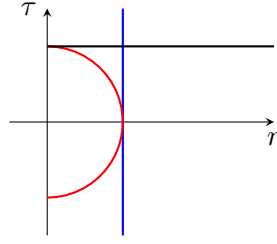
Figure 6.1.: The complex z -plane, z = r - i\tau . M^8 is a twisted product of M^6 with the right halfplane \{r > 0\} . Embedded into M^8 are the sine-cone (red half-circle), cylinder (vertical blue line), and cone (horizontal black line). M^8 is foliated either by cylinders or cones, corresponding to the foliation of the half-plane by translations of the black and blue lines. A foliation by sine-cones is obtained through variation of the radius of the red half-circle. Upon a good parametrization of the three submanifolds the G_2 -instanton equation on one of them becomes invariant under these shifts, so that a solution on a submanifold trivially extends to a Spin(7)-instanton on all of M^8 .
