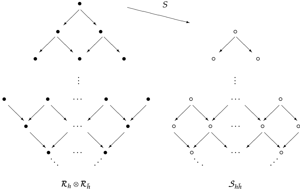
Figure 2: \mathcal{R}_h \otimes \mathcal{R}_{\bar{h}} versus \mathcal{S}_{h\bar{h}}
