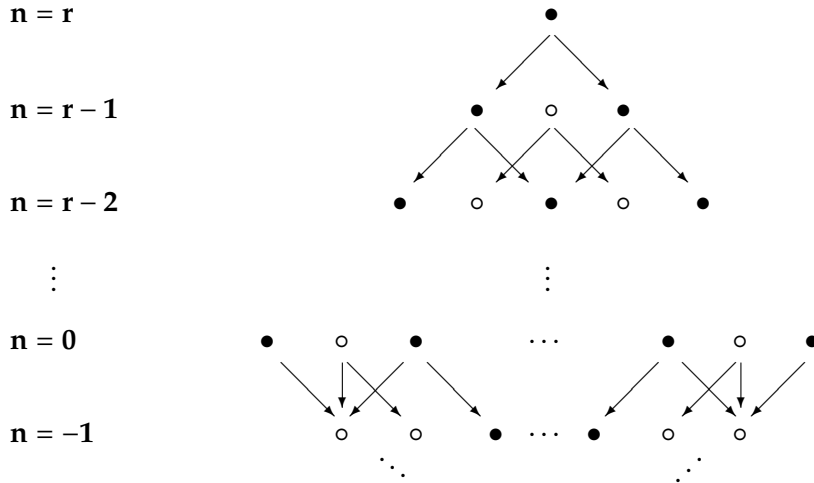
Figure 3: Comparison of \mathcal{R}_h \otimes \mathcal{R}_{\bar{h}} and \mathcal{S}_{h\bar{h}}
