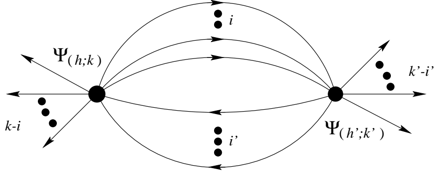
Figure 4: Graphical representation of contractions of logarithmic fields
