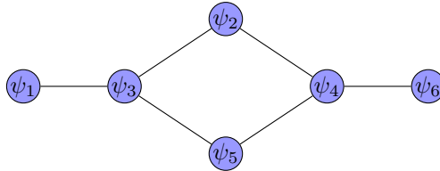
FIG. 1. A graphical representation of allowed neighbouring labels in the fusion paths of the \psi_3 anyon chain. The vertices/nodes of the graphs are the labels of anyons which are connected via an edge if and only if the two anyon labels can appear next to each other.
