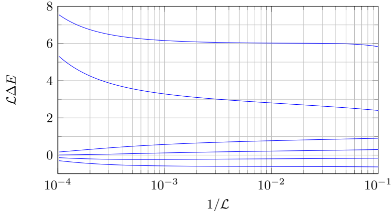
FIG. 4. \mathcal{L}\Delta E as a function of 1/\mathcal{L} for the ground state and 1st, 2nd, 3rd, 4th and 6th lowest excitations. We have omitted data for the 5th lowest excitation due to insufficient solutions of the Bethe equations. The ground state has multiplicity two with states in symmetry sectors \psi_1 and \psi_6 . The next three energies have multiplicities two, four and two, respectively, and are in sectors \psi_3 \oplus \psi_4 , \psi_2 \oplus \psi_5 and \psi_3 \oplus \psi_4 , respectively.
