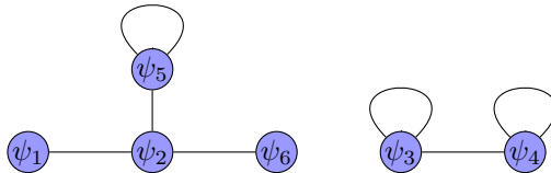
FIG. 7. The same as Figure 1 except for a chain of \psi_2 anyons.
